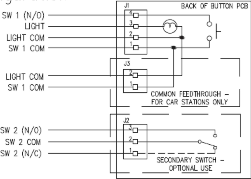
4-3-2 Style Connection Ref: DWG 10M16
